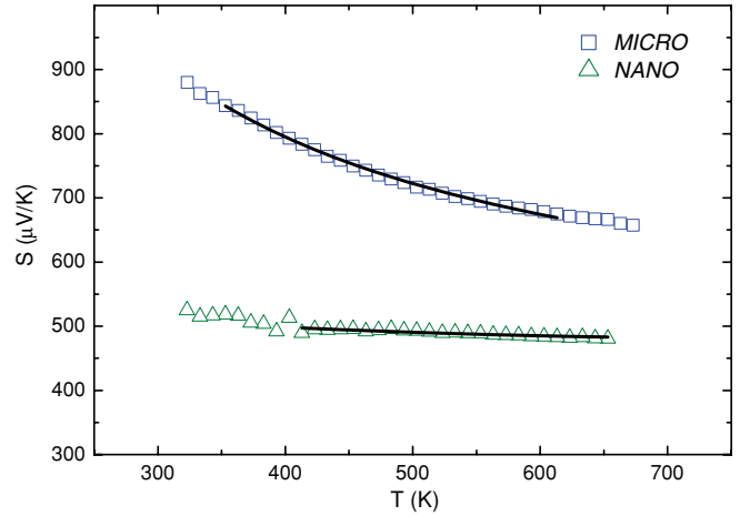
FIG. 4. (Color online) Temperature dependence of the Seebeck coefficient for the MICRO (blue, open square) and NANO (green, open triangle) \text{CuAlO}_2 samples. Solid lines are fits to Eq. (4) in the same temperature range as those of electrical conductivity (see text for details).
